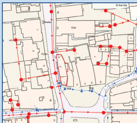
Example sewer map extract
